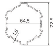
MOTOR TUBE PROFILE
