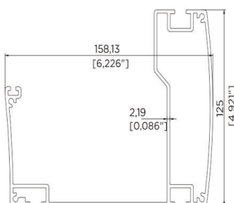
158X125 GUTTER PROFILE
