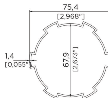
MOTOR TUBE
