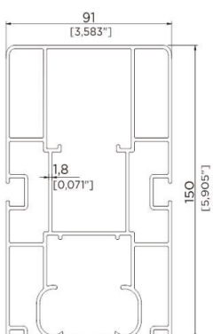
91X150 RAL PROFILE
