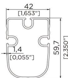
42X59,7 FABRIC SUPPORT PROFILE
