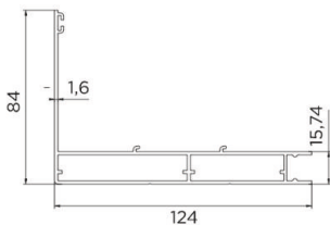
SIDE RAIL PROFILE
