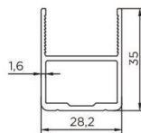
24MM GLASS FRAME PROFILE
