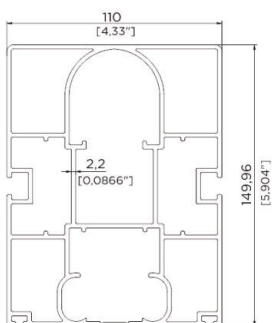
110X150 RAIL PROFILE
