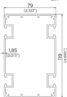
HORIZONTAL PROFILE
