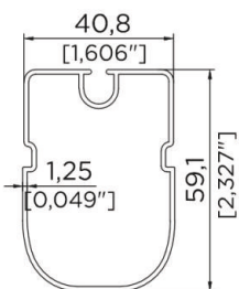
40,8X59,1 FABRIC SUPPORT PROFILE
