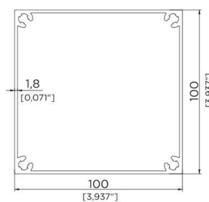
100X100 PILAR PROFILE
