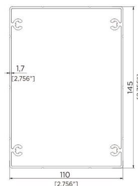
110X145 PILLAR PROFILE
