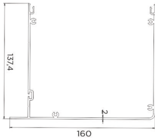
MOTOR BOX PROFILE
