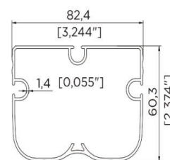
82,4X60,3 FABRIC SUPPORT PROFILE
